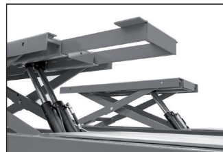
Extending lift table.
